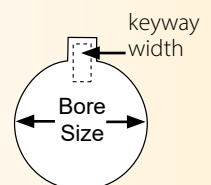
Keyway Broach Shim
